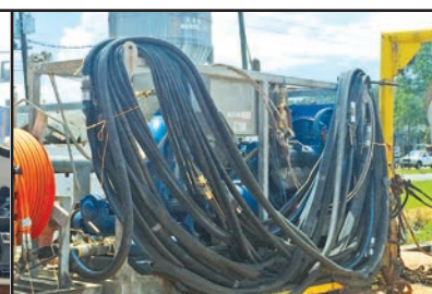
6 x 6 Jet Pump w/ Jet Hose
