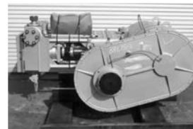
FMCWT2450 Pump 4.5 FLUID END WT2450, Part# P540619, 2400HP, Speed 1950, Gear Ratio: 6:39:1 - $110,000
