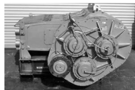
SPM 3000 HP Pump BAS3000, G0214-10000 3000BHP, 12 Stroke, 7.68 Gear Ration, MFG 2/2014, *No Fluid End - $295,000
