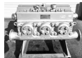
Pacemaker Pumps 700BHP BS# 322656, 141111PTL7/576 Fluid End BSPAR# 322690 SN: F0914-25960, MFG 2014 $105,000
